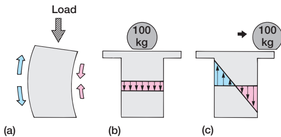
FIGURE 4.36 Loading. (a) When a material bends under a load, compressive forces (solid arrows) develop along the concave side, tensile forces (open arrows) along the convex side. (b) When a supportive column is loaded symmetrically (with the weight centered), the only type of force experienced is compressive force. The distribution of the 100-kg mass within a representative section is depicted graphically. The lengths of the down arrows show equal distribution of compressive forces within this representative section. (c) Asymmetrical loading of the same mass causes the column to bend. The column experiences compressive forces (down arrows) and tensile forces (up arrows). Both compressive and tensile forces are greatest near the surface and least toward the center of the column.
