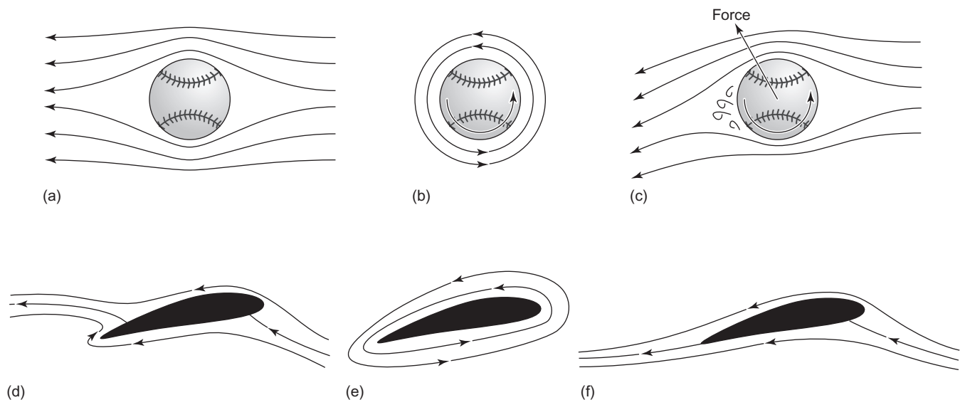
FIGURE 9.52 Aerodynamic circulation. Curve ball. A baseball in flight may experience two airflow patterns as a consequence of its motion. (a) Without rotation, the air flows symmetrically across both sides. (b) With rotation, the ball pulls the air near its surface, producing a bound, thin, circulating layer. (c) Added together, flow is speeded up on one side, slowed on the other, producing deflection of the overall airstream and an unbalanced force on the ball that causes it to curve. Lift of an airfoil. An airfoil does not spin, but its effect on airflow can be similar. (d) Airflow without circulation; (e) circulation only; (f) total, actual flow pattern around an airfoil.
