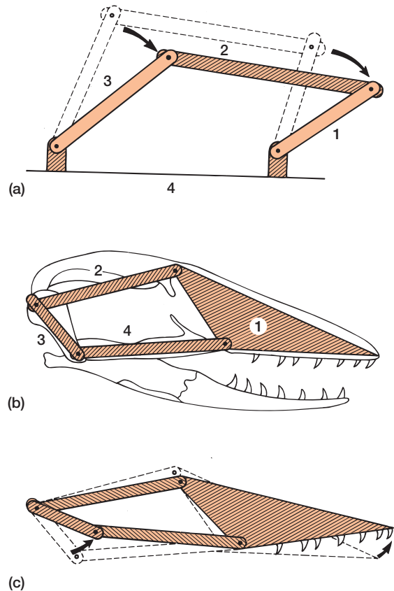
FIGURE 4.32 Kinematic chain. (a) This four-linkage mechanism is joined by pin connections so that the motion of link 3 imparts a specific motion to the three other links. (b) The four-linkage chain of a lizard skull (ignoring the lower jaw) is constrained. (c) Again, motion of link 3 imparts a specific motion to each of the other links.
